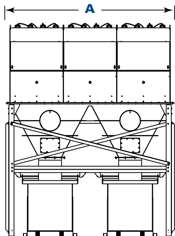
CPC-3, -4 Side View
