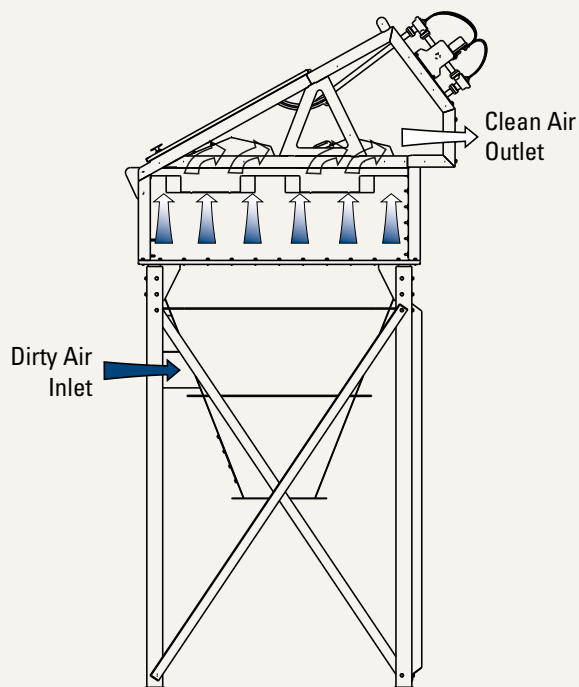
Normal Operation for CPC-3 through CPC-48 Models
